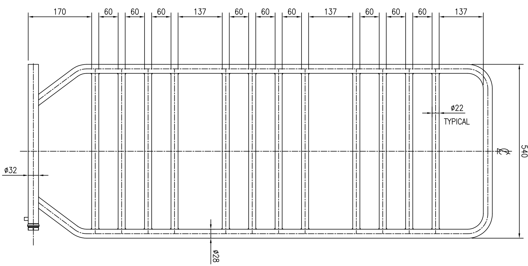
FRONT ELEVATION
